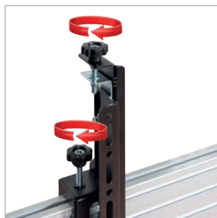
Micro-adjustment arms feature tool-less height and depth adjustment knobs
